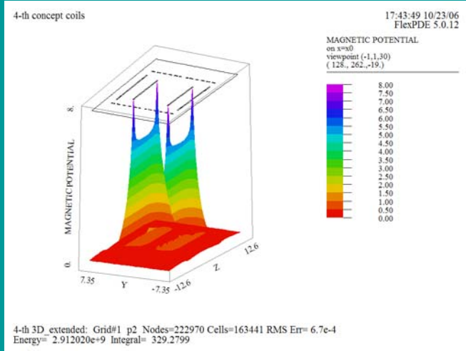
Magnetic potential
